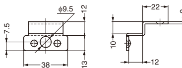
Strike for overlay door (sold separately)
