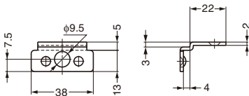
Strike for inset door (included)
