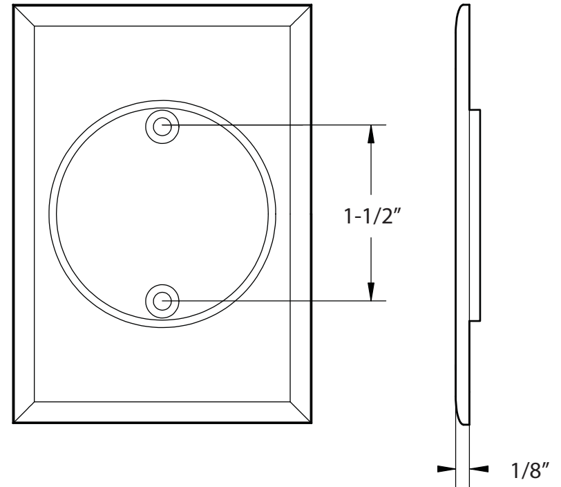
RECTANGULAR TUBULAR POCKET PASSAGE, INSIDE TRIM
