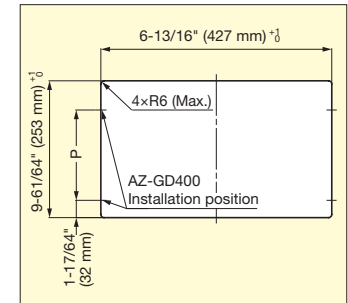
AZ-GD400-HL
