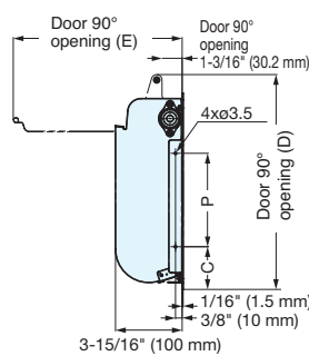
AZ-GD310-HL
