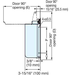
AZ-GD400-HL
